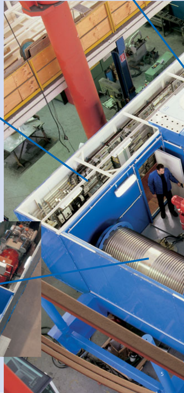
Superstructure with individual rooms, designed as modules
